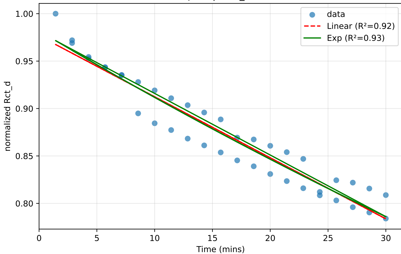
Chip 37 | 1nM_disso
