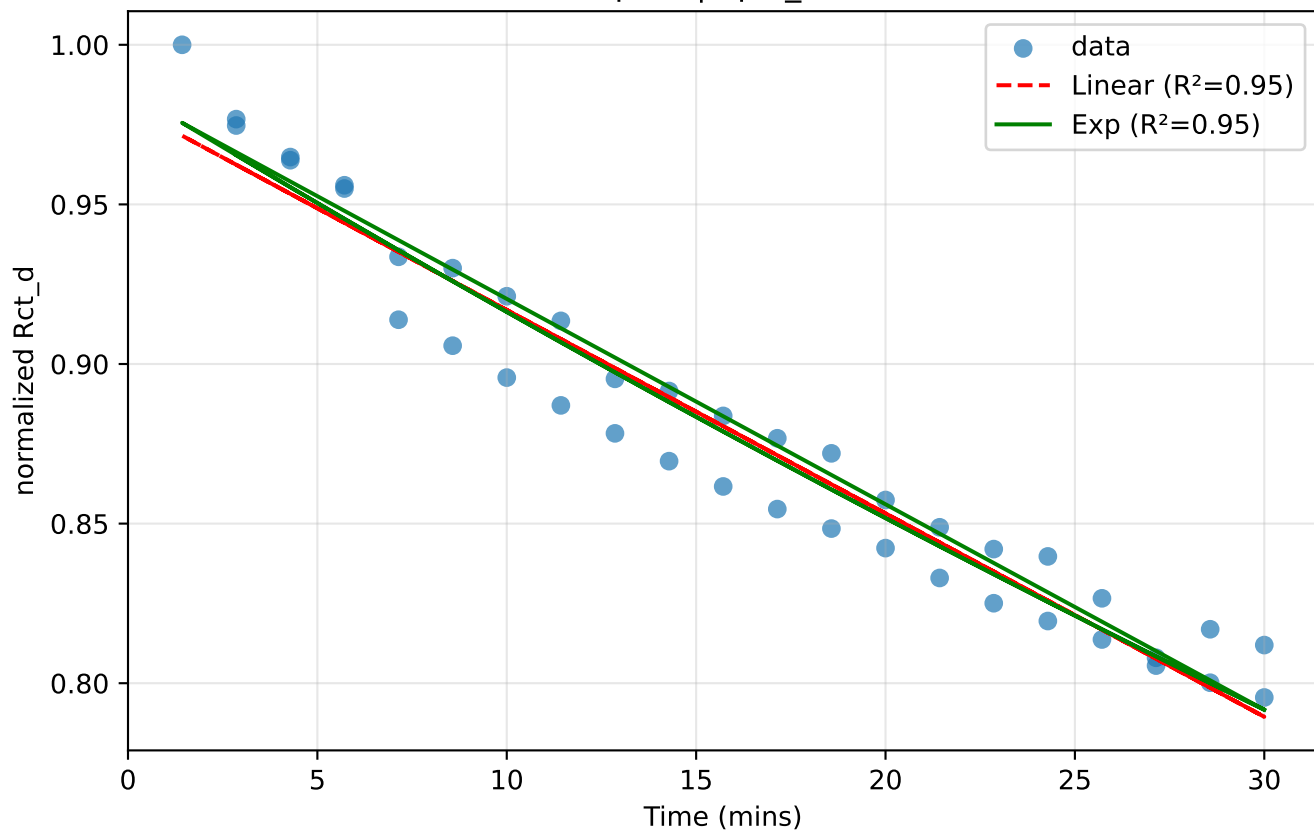
Chip 37 | 0pM_disso
