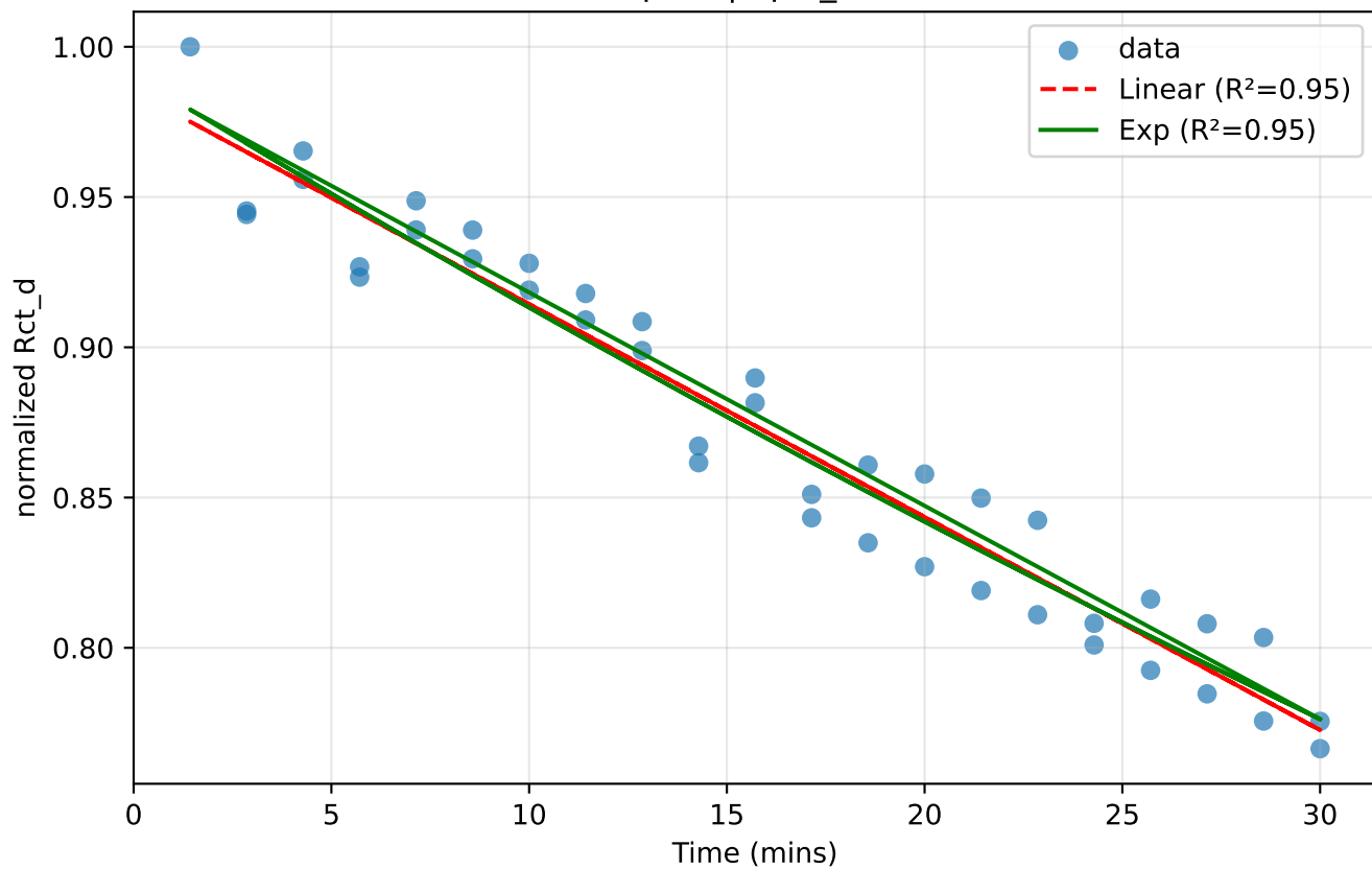
Chip 39 | 0pM_disso
