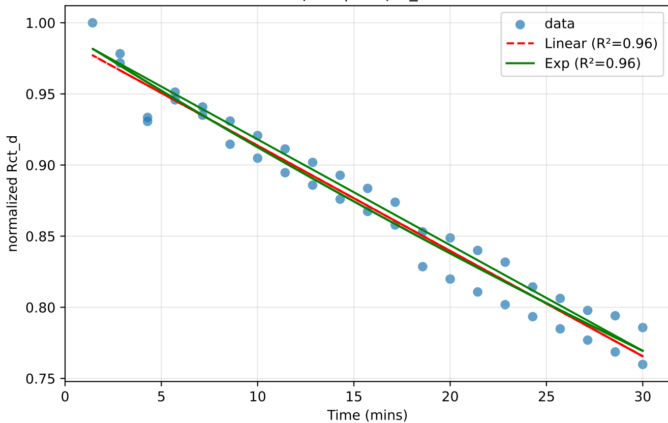
Chip 39 | 100pM_disso
