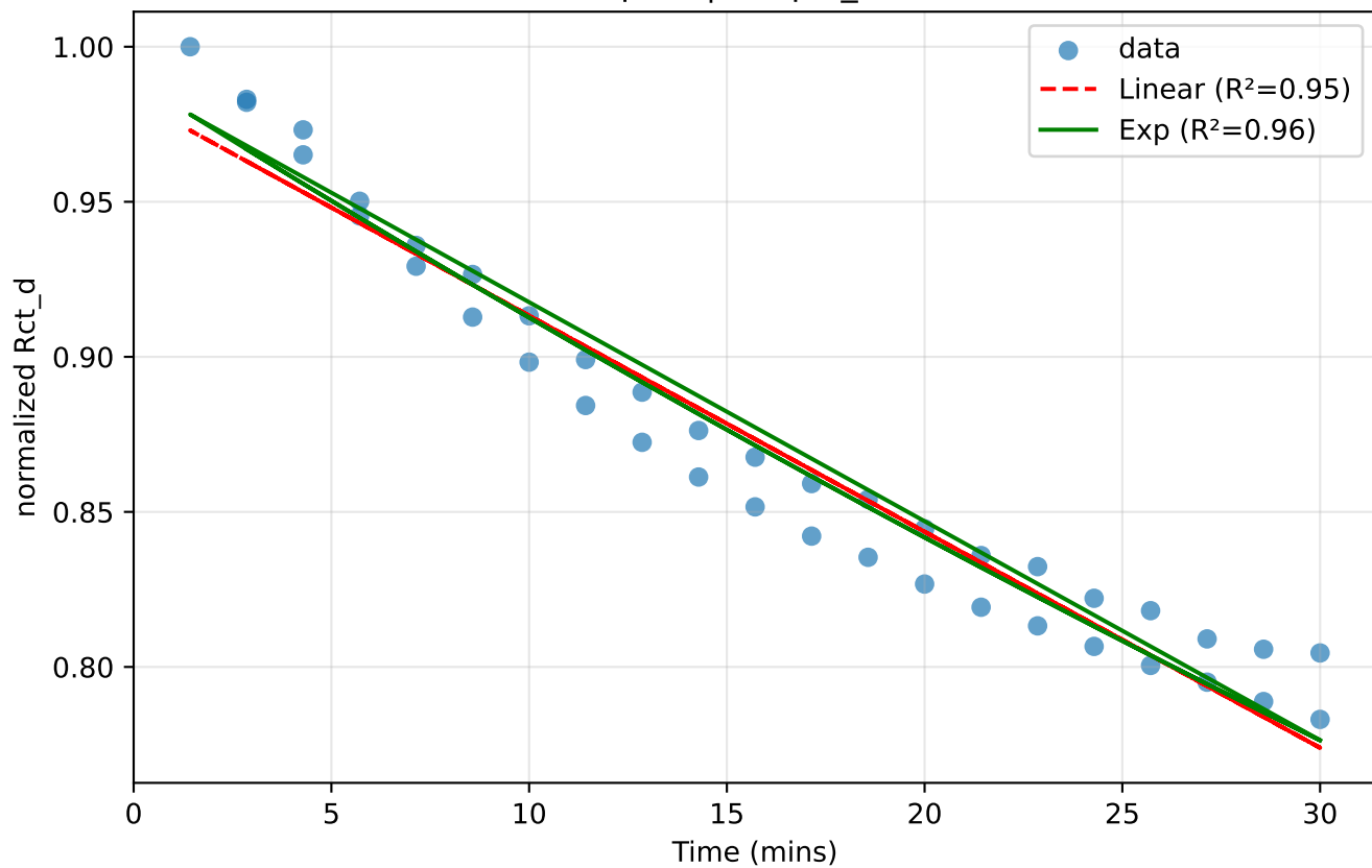
Chip 40 | 100pM_disso
