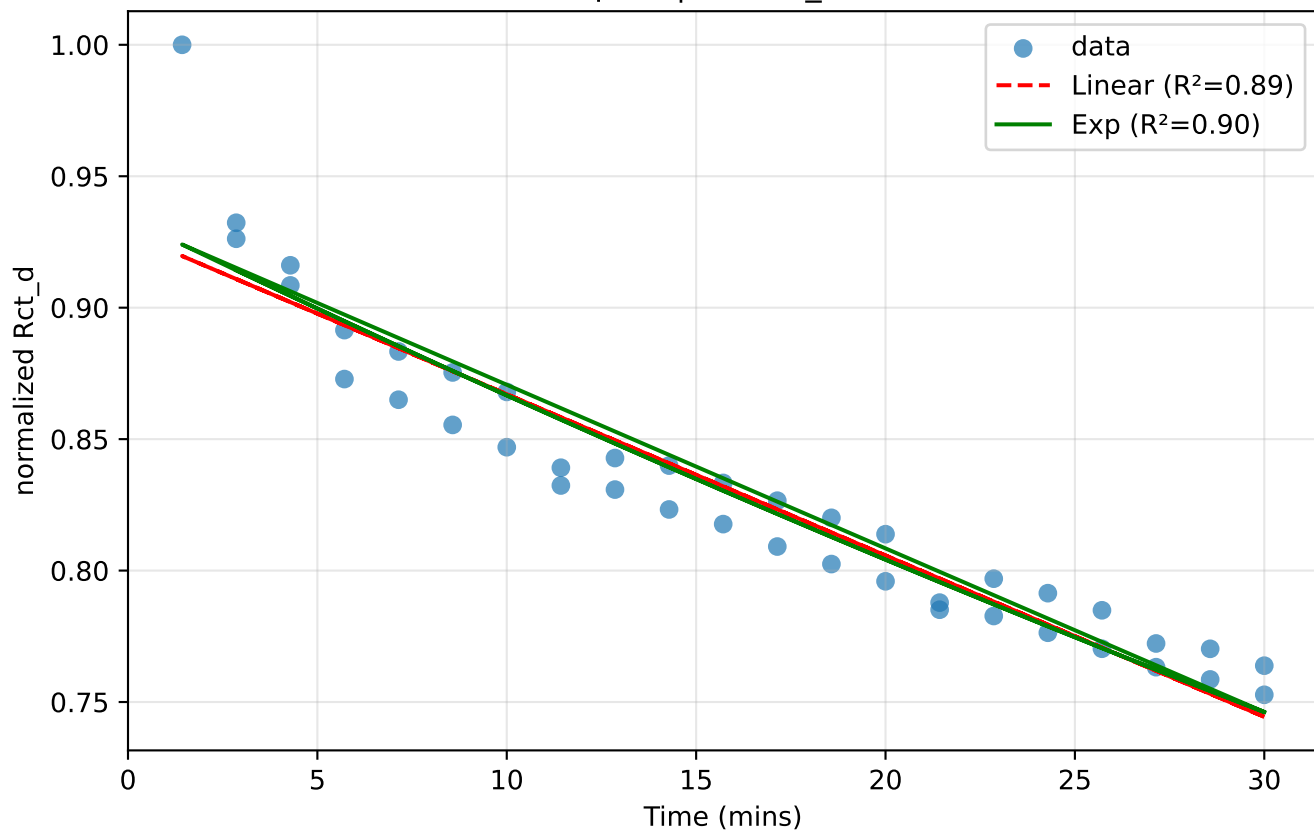
Chip 37 | 100nM_disso
