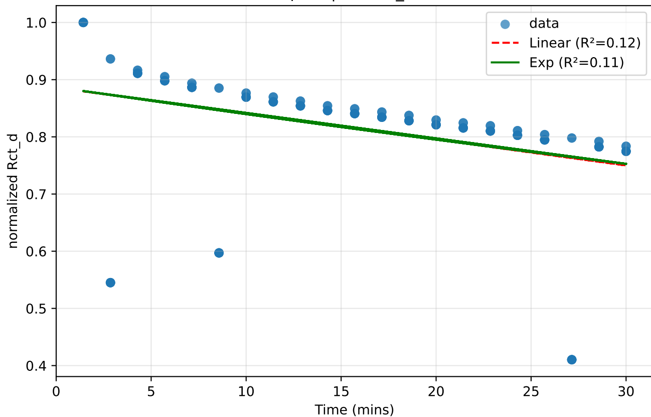
Chip 46 | 100nM_disso
